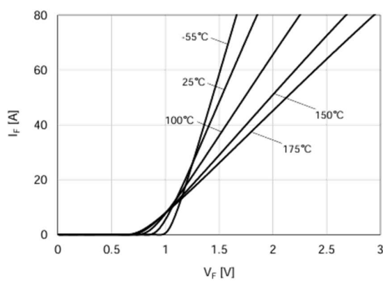
Figure 3 Forward Characteristics
