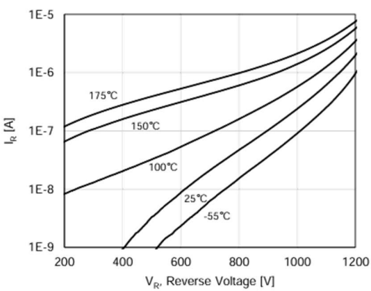
Figure 4. Reverse Characteristics
