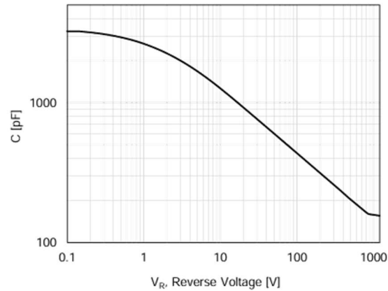
Figure 7. Capacitance Characteristics
