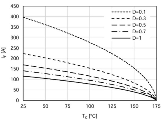
Figure 2. Current Derating
