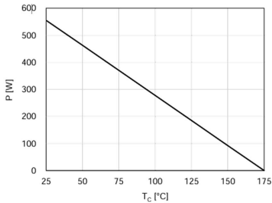
Figure 1. Power Derating
